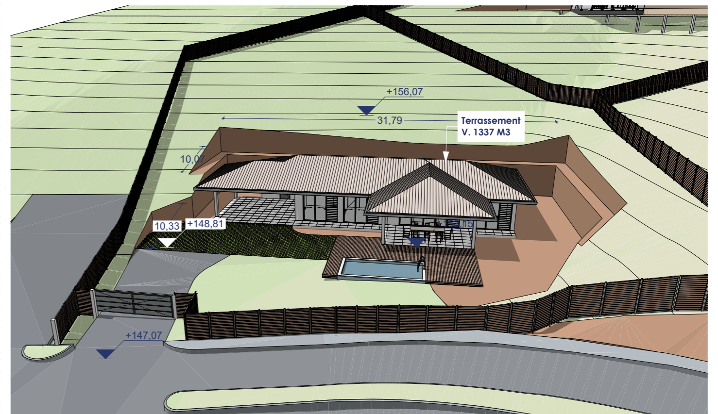
OP-3D9 Perspective L44 1:200
